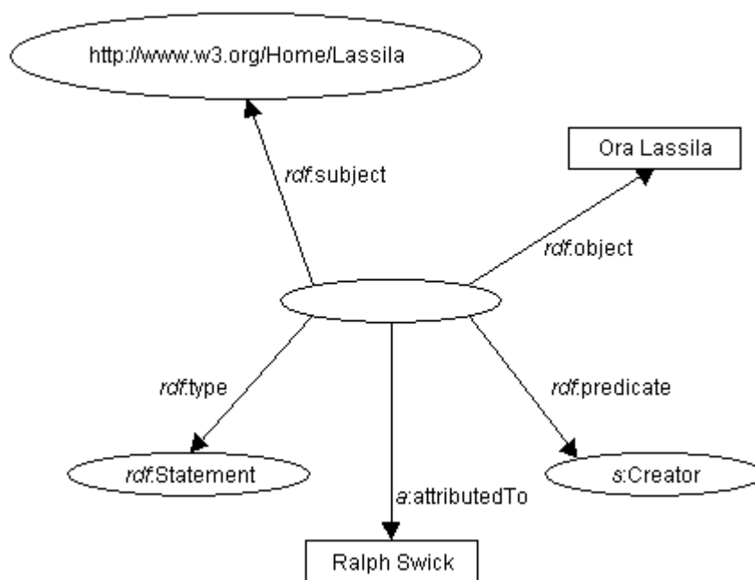
Figure 8: Representation of a reified statement
