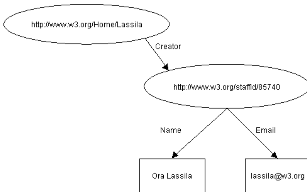
Figure 3: Structured value with identifier
