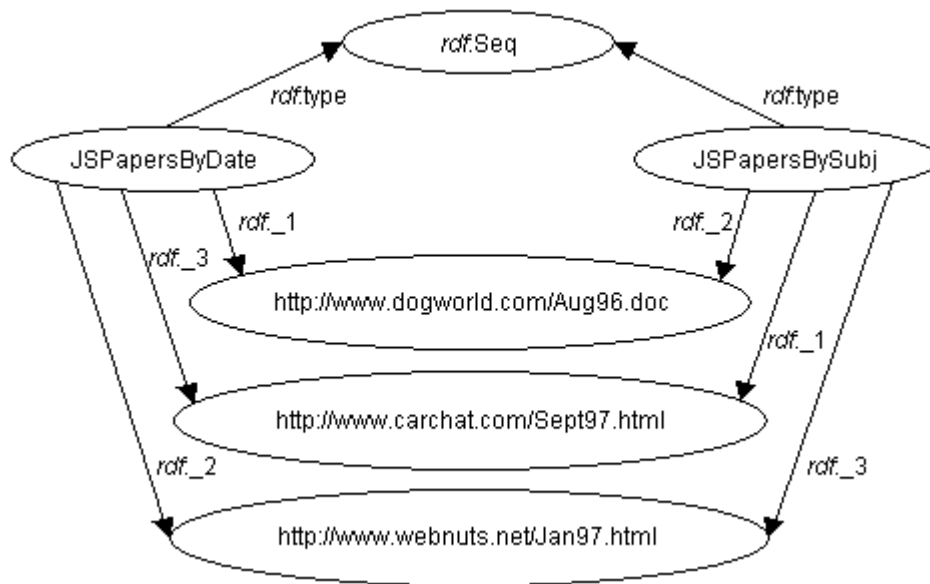
Figure 13: Sharing values between two sequences
