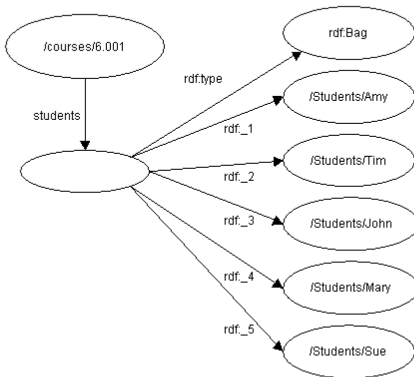
Figure 4: Simple Bag container
