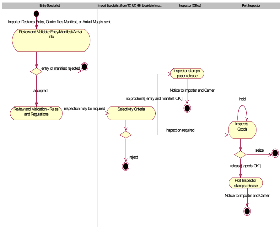
Figure 25. UML Business Activity Model
