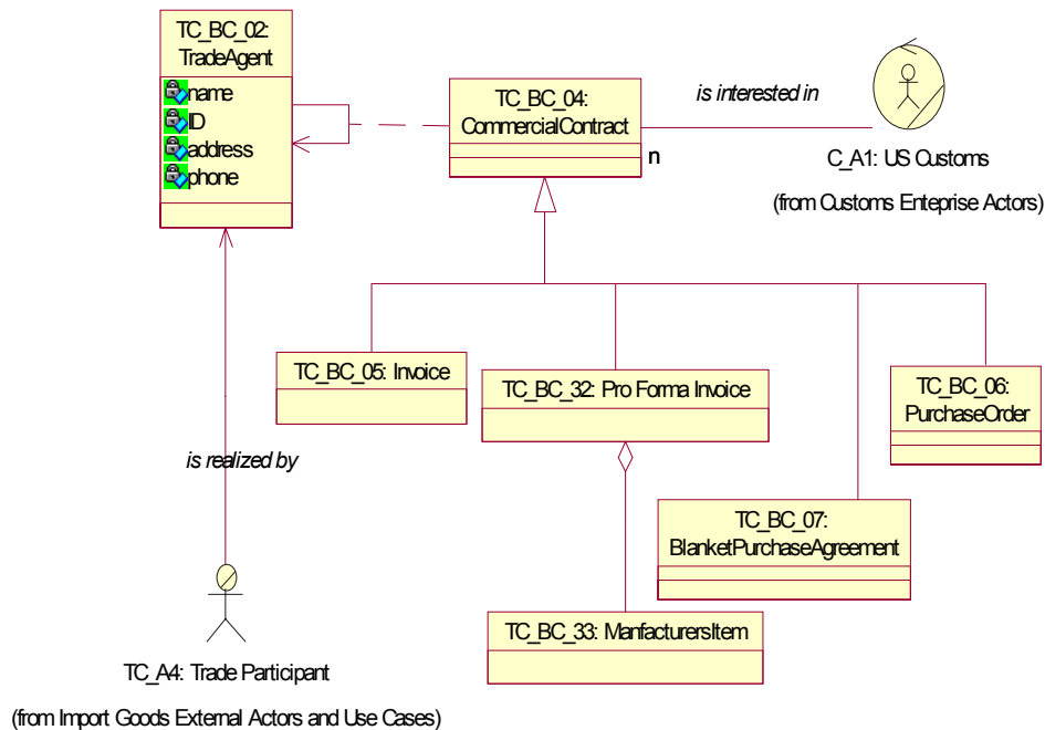
Figure 29. UML Business Class Diagram, Trade Class Model (Commercial View)
