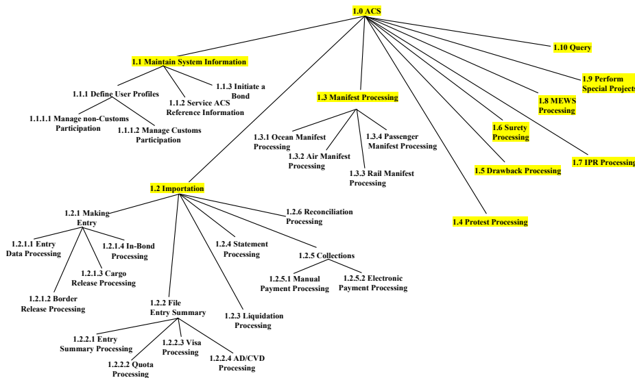
Figure 24. Activity Tree, U.S. Customs Service Automated Commercial System Activity Tree
