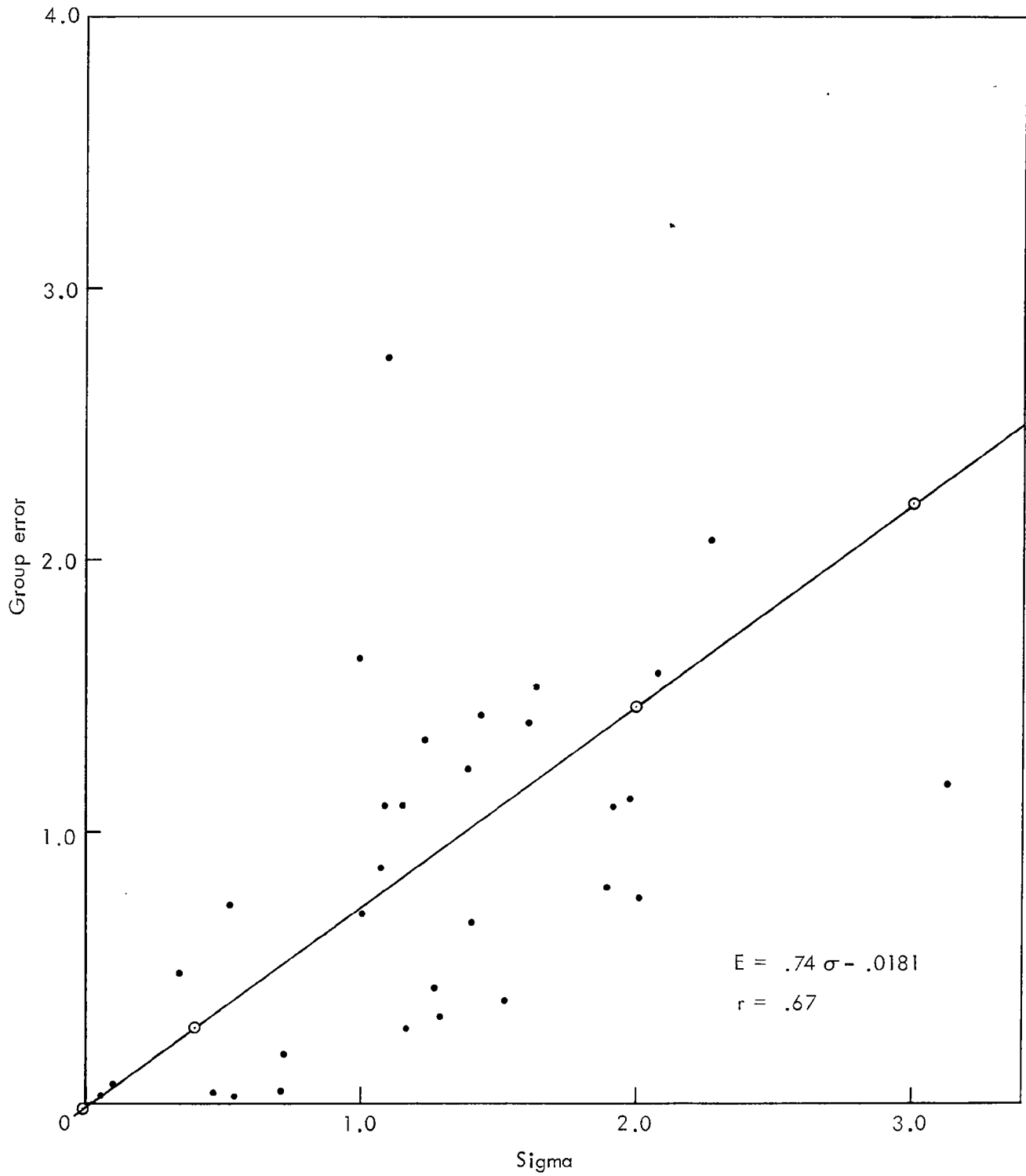
Fig. 1—Round 1 group error versus standard deviation
