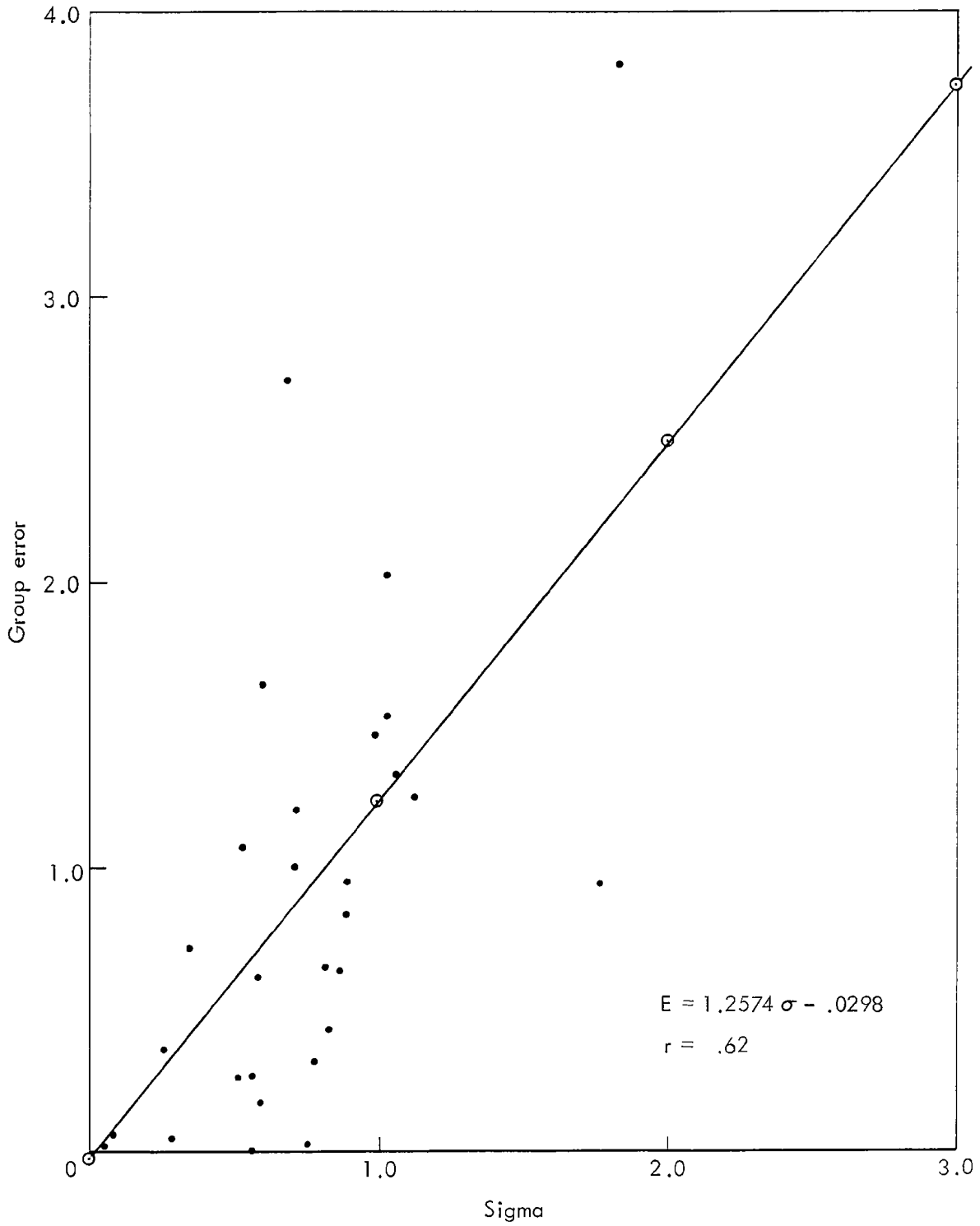
Fig. 2—Round 2 error versus standard deviation
