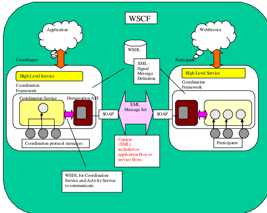
Figure 18, WS-CF components.
