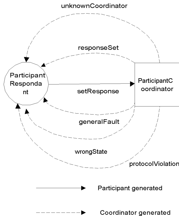
Figure 5, Participant-to-coordinator interactions.
